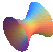
One-sheet hyperboloid
