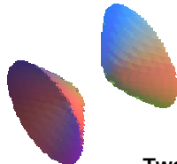
Ellipsoid
