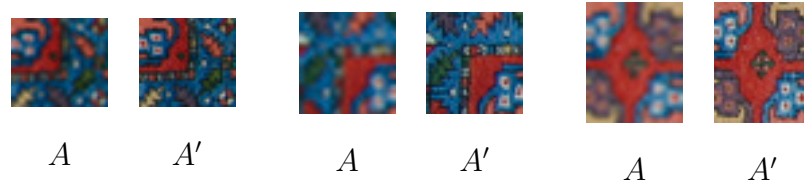
Training pairs
